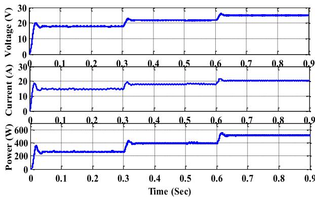
FIGURE 14. Wind system output voltage, current, and power at different wind velocity levels.
