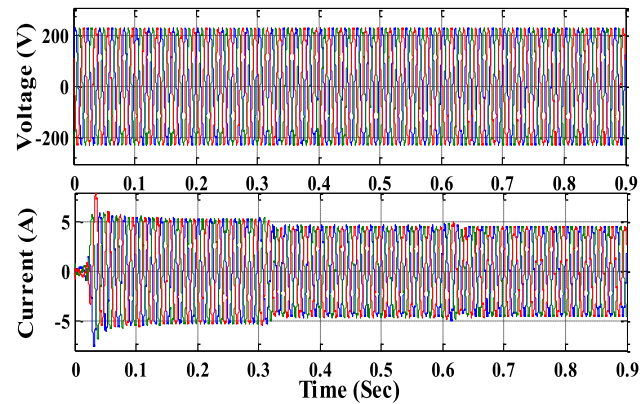
FIGURE 17. Inverter voltage, current.
