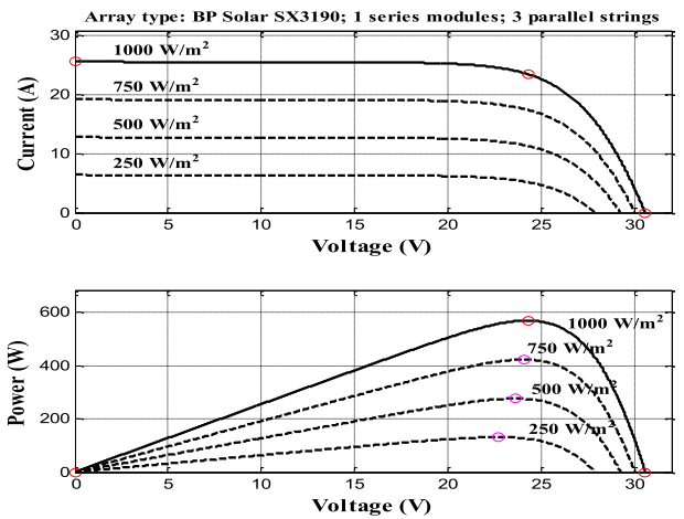
FIGURE 4. I-V and P-V characteristics of BP solar SX3190 model.
