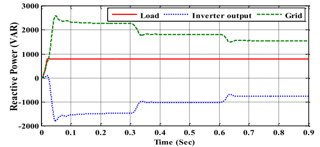
FIGURE 21. Reactive power.
