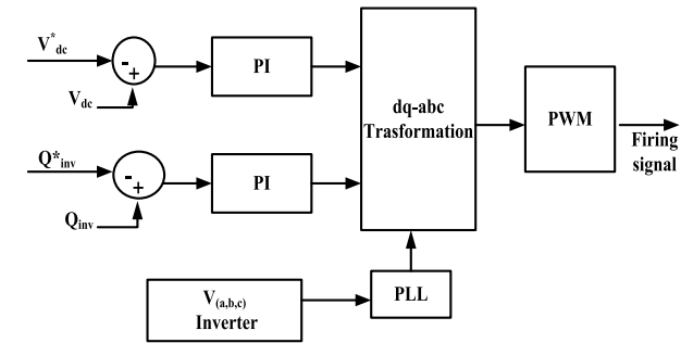
FIGURE 16. Grid side current regulated controller.
