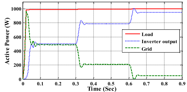
FIGURE 20. Active power.
