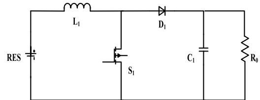
FIGURE 6. Equivalent circuit of conventional boost converter.
